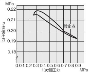
R151
