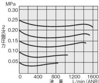
R301
