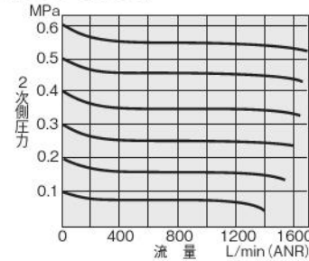
R300・R302
