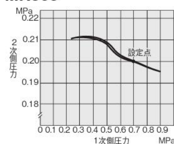
MR303
