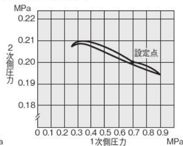
R300・R302
