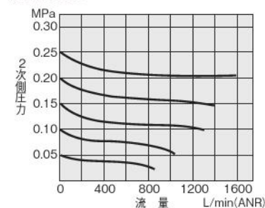
MR303
