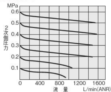
MR302
